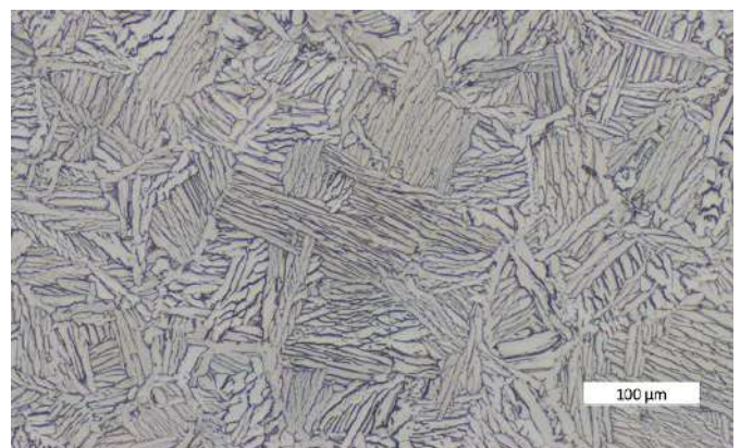
HIP: 820 °C; 2000 bar; 2 h
